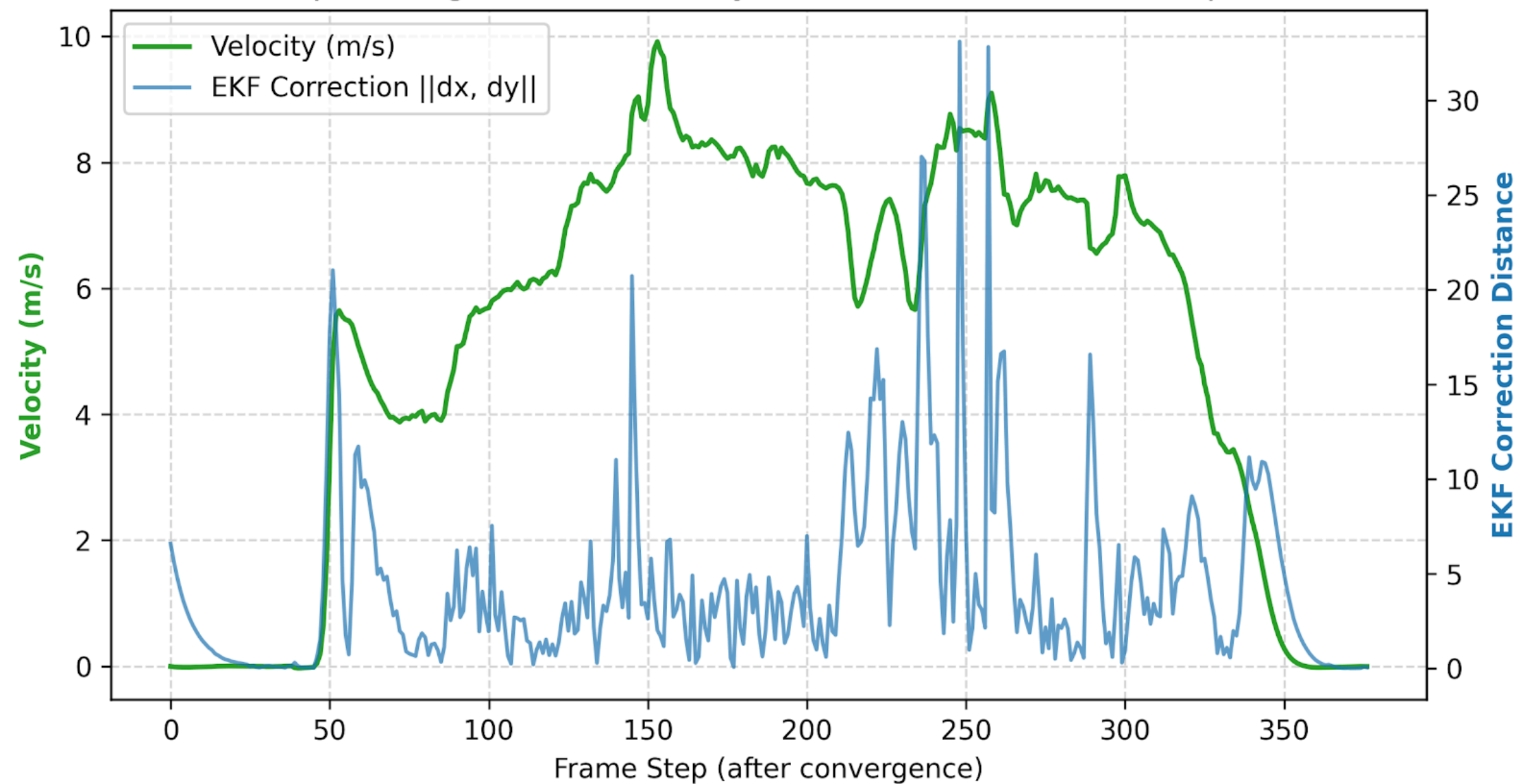
Temporal Alignment of Velocity Peaks and EKF Correction Spikes
